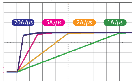
Ch4 load current 20A/div Horizontal 10us/div
